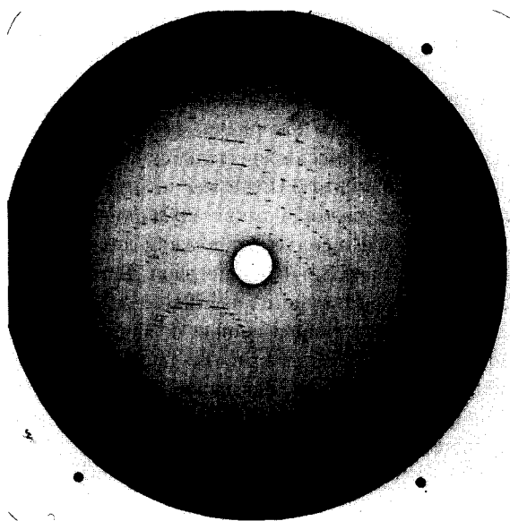
Fig. 1. A rotation photograph of a crystal of H50S, obtained at 90 K at station F1/CHESS, operating at 5.3 GeV and 50 mA. Crystal-to-film distance = 220 mm, collimator = 0.1 mm; wave length = 0.9091 Å.
