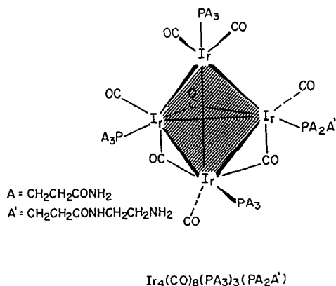
Fig. 2. Schematic representations of the undecagold and the tetrairidium clusters [12,13,26].
