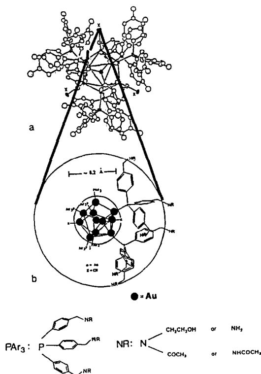
Fig. 2. Schematic representations of the undecagold and the tetrairidium clusters [12,13,26].
